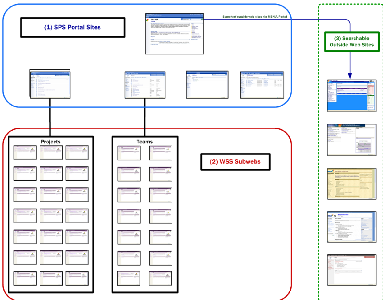
Figure 1: Logical model of Fox portal architecture
